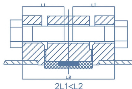
Bolt Connection of Lug Butterfly Valve
